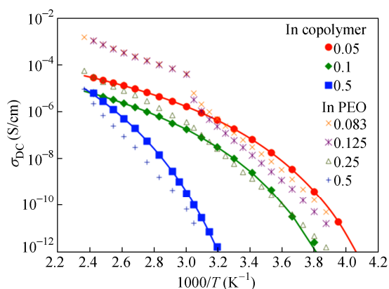
Fig. 6 DC conductivity \sigma_{DC} versus 1000/T for the BBP/LiTf samples of r = 0.05 , 0.1 , and 0.5 (For comparison, the reported \sigma_{DC} data of PEO/LiTf mixtures are added [41] ). Curves are fitted with VFT equation \sigma_{DC} = \sigma_0 \exp[-B/(T - T_0)] .
